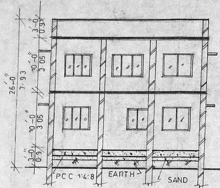
SECTION ON P.Q
