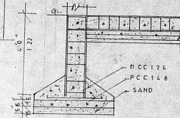
FOUNDATION DETAIL
